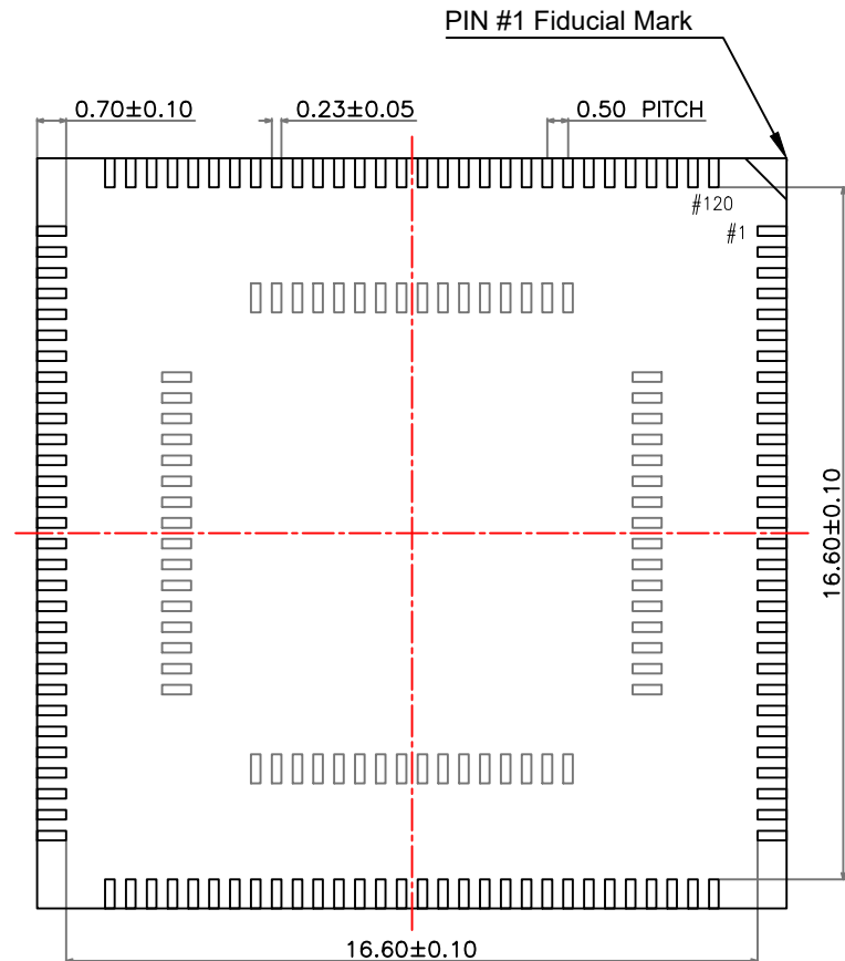
BOTTOM VIEW
